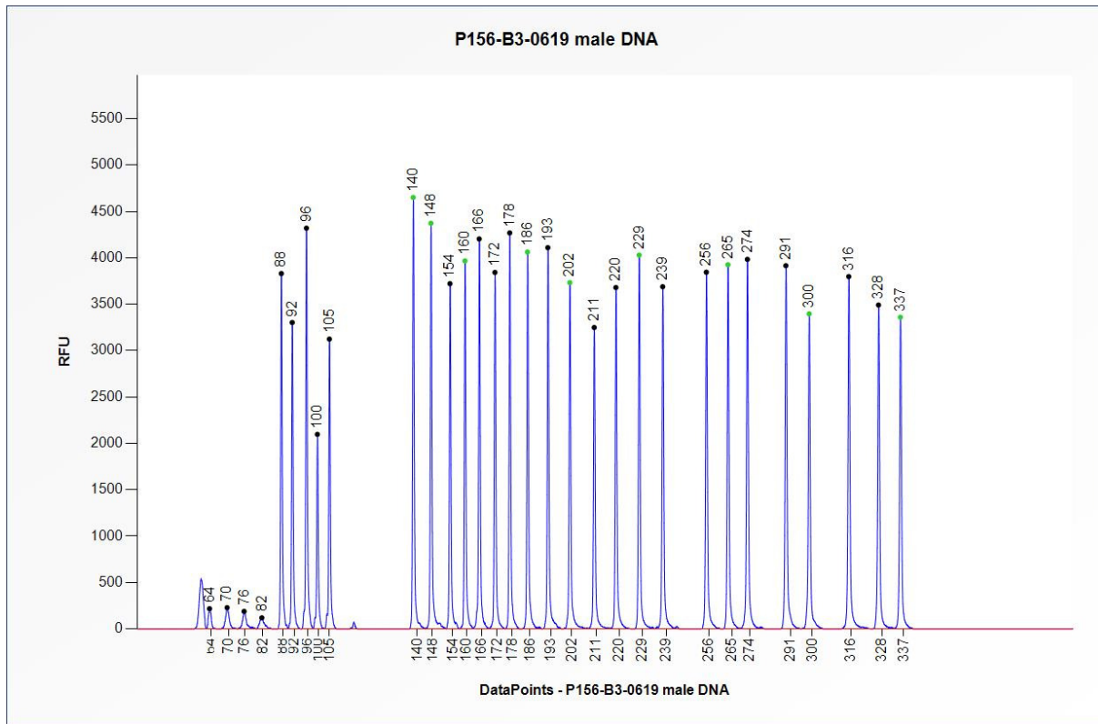
Figure 1. Capillary electrophoresis pattern from a sample of approximately 50 ng human male control DNA analysed with SALSA MLPA Probemix P156 GALT (B3-0619).
