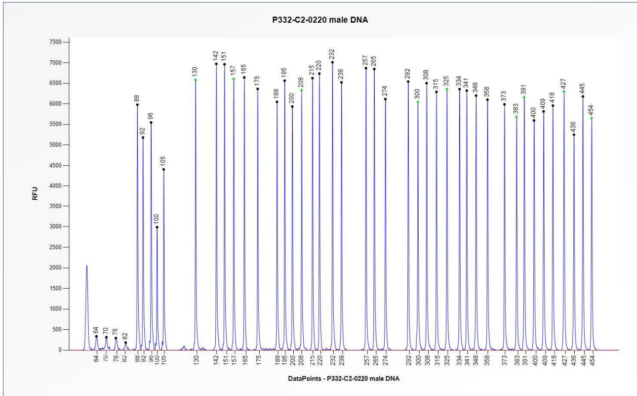
Figure 1. Capillary electrophoresis pattern from a sample of approximately 50 ng human male control DNA analysed with SALSA MLPA Probemix P332 COL5A1 MIX-2 (C2-0220).
