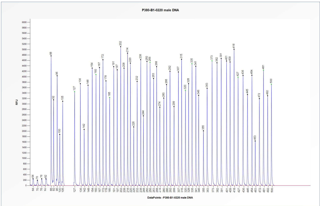
Figure 1. Capillary electrophoresis pattern from a sample of approximately 50 ng human male control DNA analysed with SALSA MLPA Probemix P380-B1 Wilms' tumour (B1-0220).
