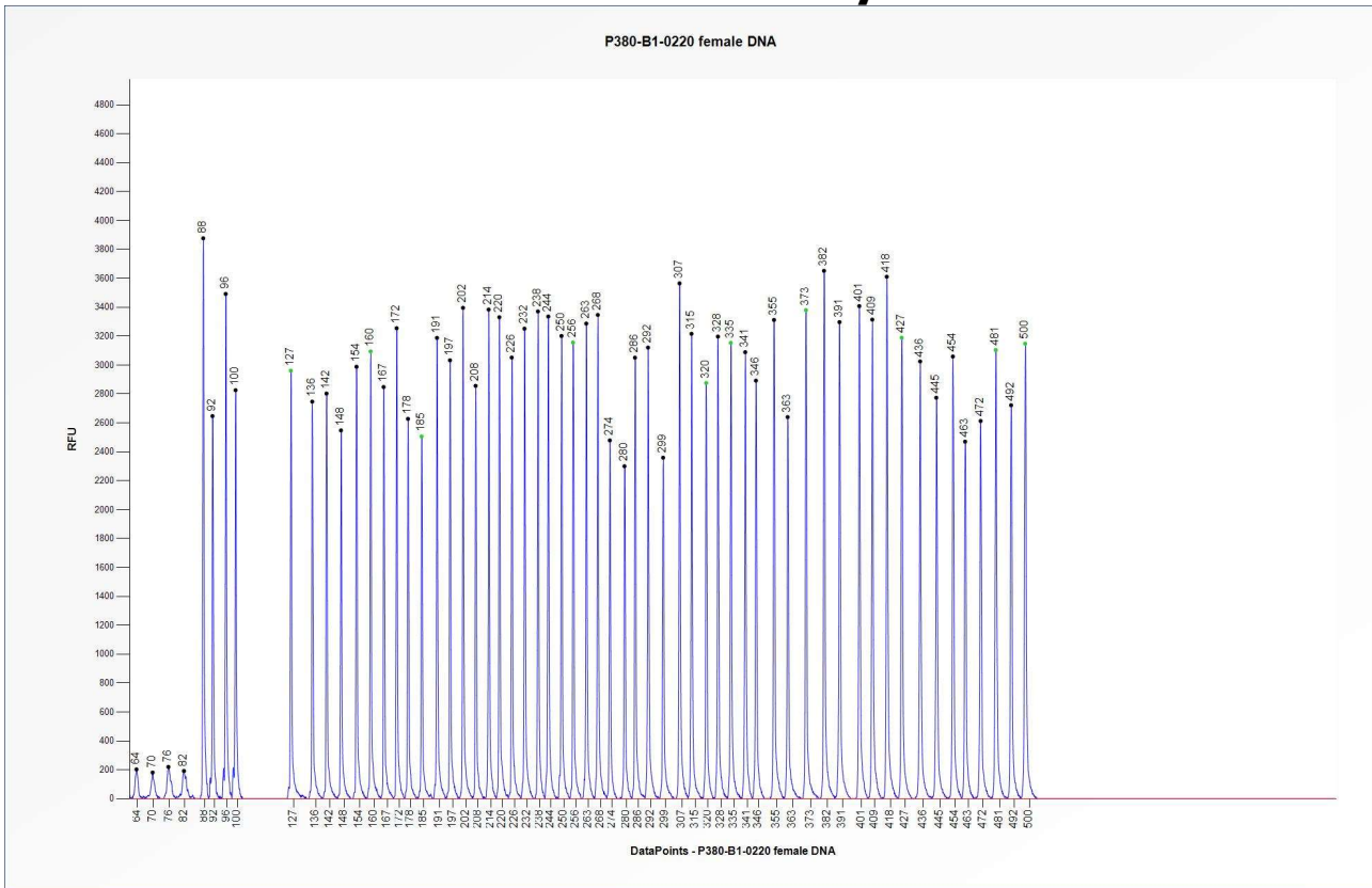
Figure 2. Capillary electrophoresis pattern from a sample of approximately 50 ng human female control DNA analysed with SALSA MLPA Probemix P380-B1 Wilms' tumour (B1-0220).
