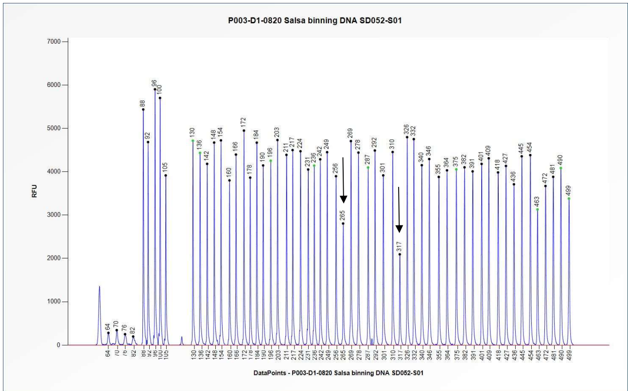
Figure 2. Capillary electrophoresis pattern from SALSA Binning DNA SD052-S01 (approximately 50 ng) analysed with SALSA MLPA Probemix P003 MLH1/MSH2 (D1-0820). The location of the inversion probes at 265 and 317 nt is indicated.
