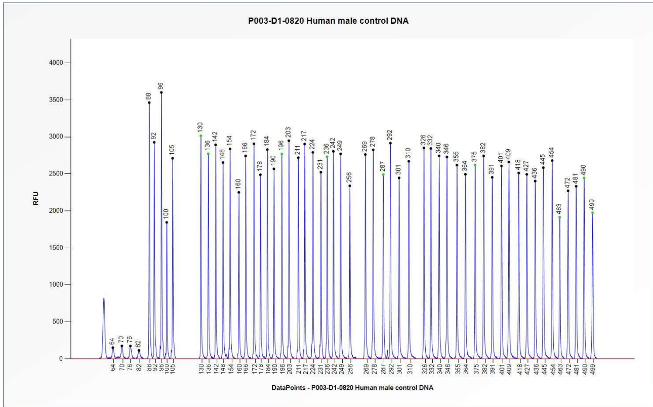
Figure 1. Capillary electrophoresis pattern from a sample of approximately 50 ng human male control DNA analysed with SALSA MLPA Probemix P003 MLH1/MSH2 (D1-0820).
