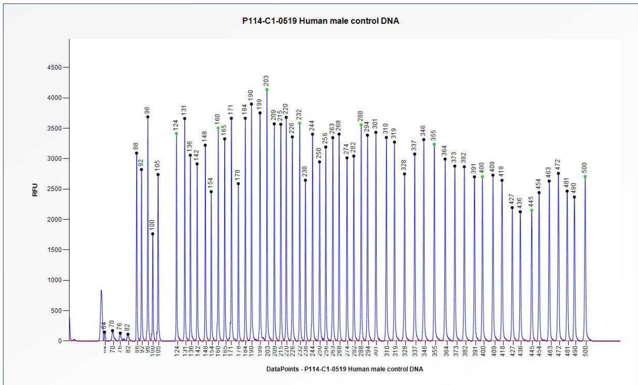
Figure 1. Capillary electrophoresis pattern from a sample of approximately 50 ng human male control DNA analysed with SALSA MLPA Probemix P114 Long-QT (C1-0519).
