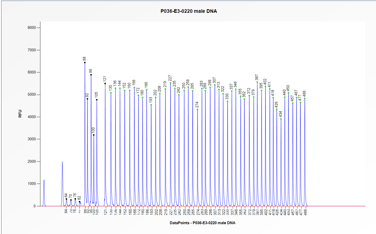
Figure 1. Capillary electrophoresis pattern from a sample of approximately 50 ng human male control DNA analysed with SALSA MLPA Probemix P036 Subtelomeres Mix 1 (E3-0220).
