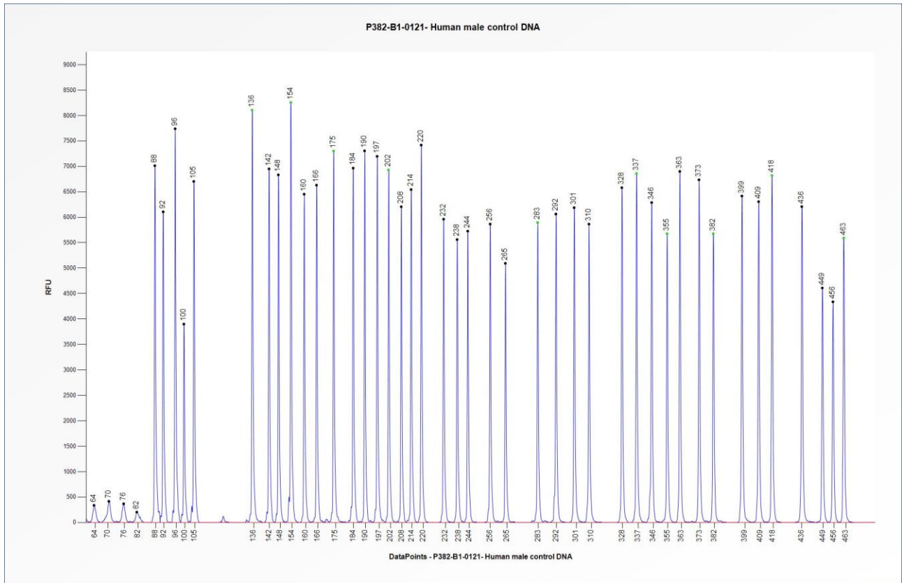
Figure 1. Capillary electrophoresis pattern from a sample of approximately 50 ng human male control DNA analysed with SALSA MLPA Probemix P382 COL11A1 mix 2 (B1-0121).
