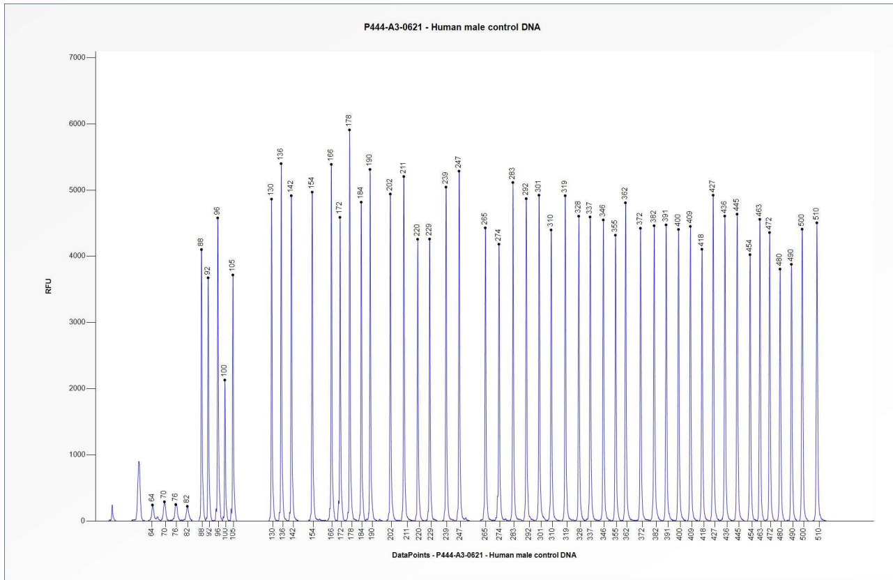
Figure 1. Capillary electrophoresis pattern from a sample of approximately 50 ng human male control DNA analysed with SALSA MLPA Probemix P444 COL4A4 (A3-0621).
