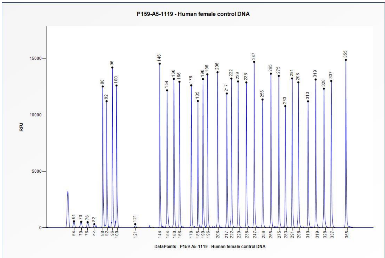
Figure 2. Capillary electrophoresis pattern from a sample of approximately 50 ng human female control DNA analysed with SALSA MLPA Probemix P159 GLA (A5-1119).
