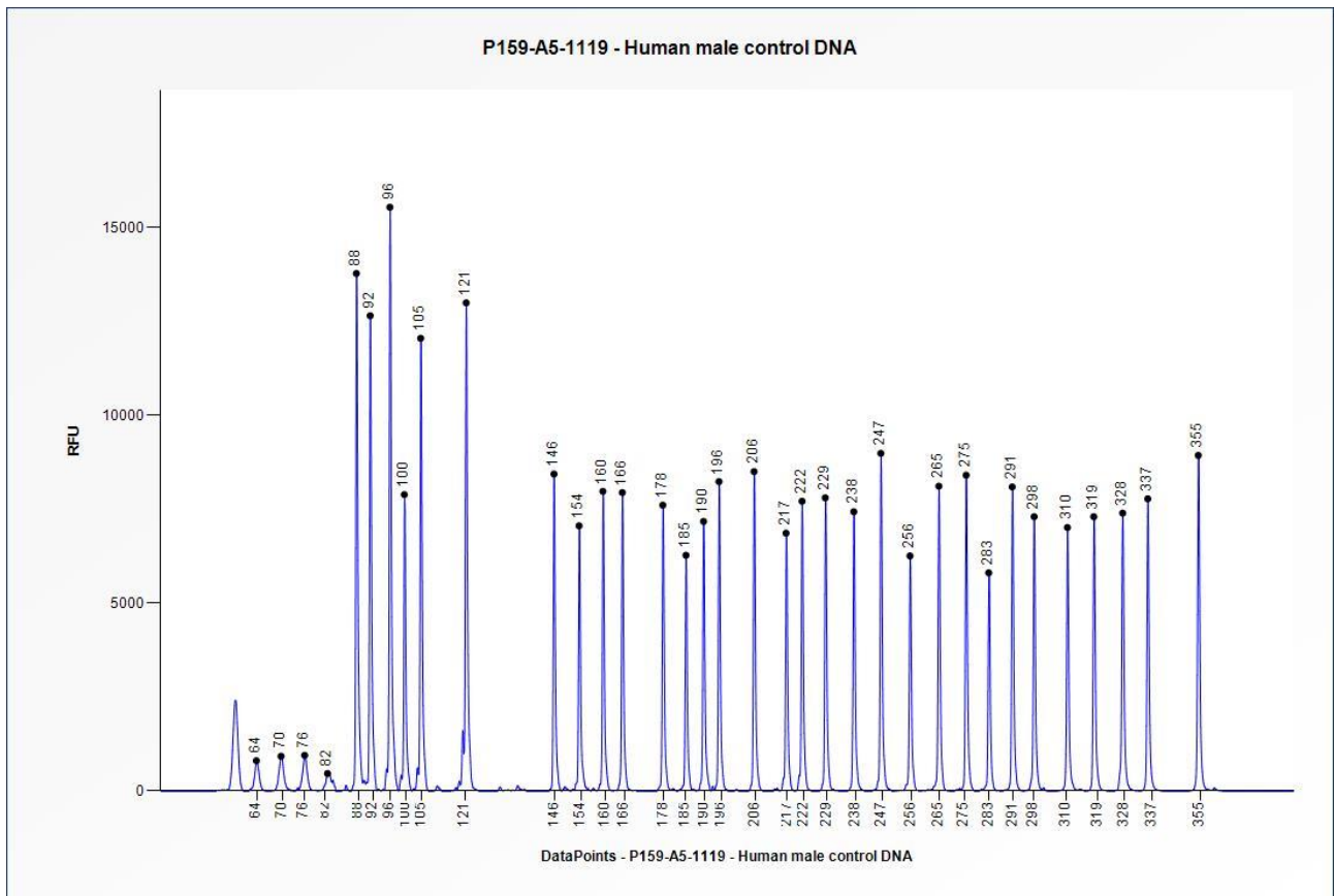
Figure 1. Capillary electrophoresis pattern from a sample of approximately 50 ng human male control DNA analysed with SALSA MLPA Probemix P159 GLA (A5-1119).
