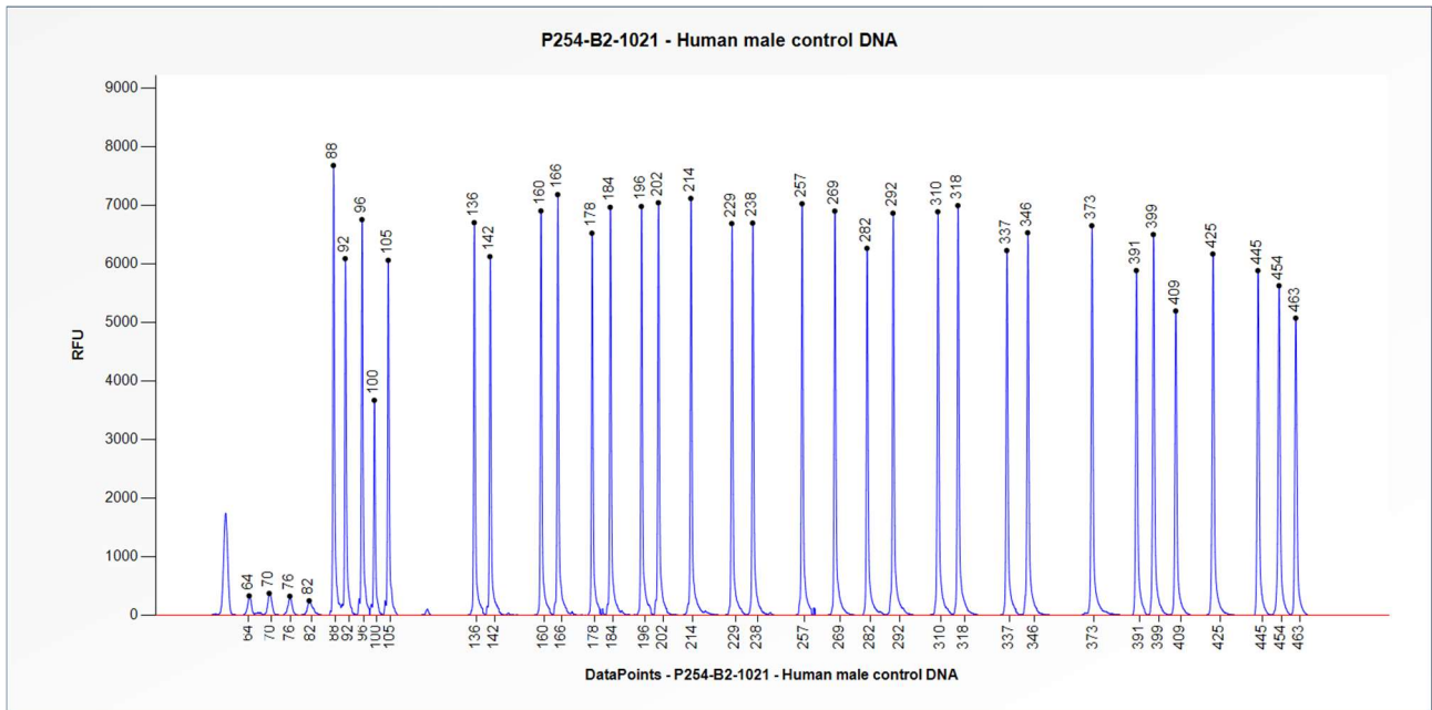
Figure 1. Capillary electrophoresis pattern from a sample of approximately 50 ng human male control DNA analysed with SALSA MLPA Probemix P254 PSEN1 (B2-1021).
