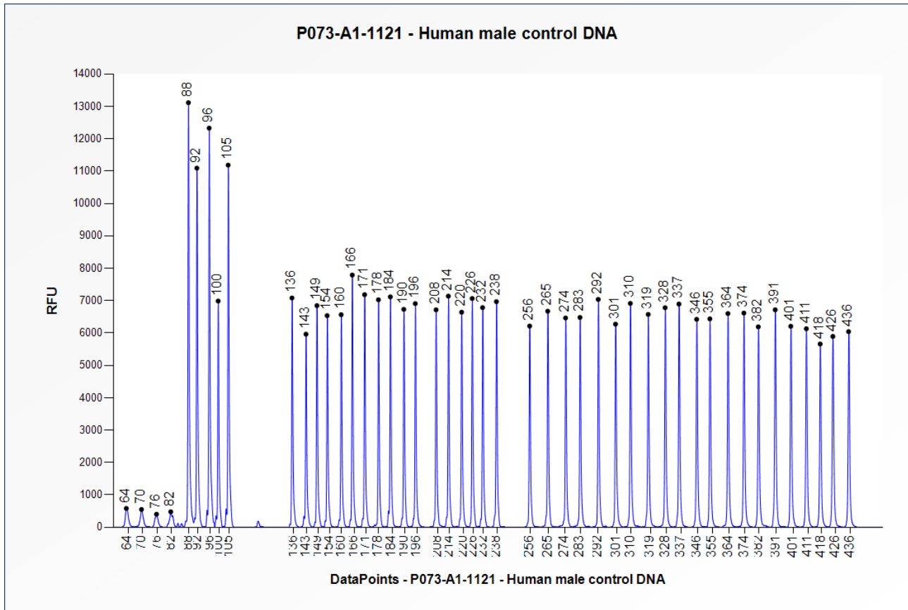
Figure 1. Capillary electrophoresis pattern from a sample of approximately 50 ng human male control DNA analysed with SALSA MLPA Probemix P073 IKBKG (A1-1121).
