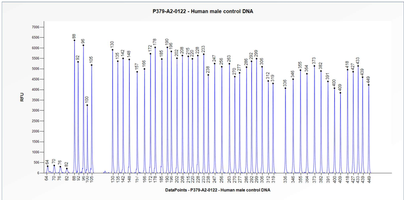
Figure 1. Capillary electrophoresis pattern from a sample of approximately 50 ng human male control DNA analysed with SALSA MLPA Probemix P379 NRXN1 (A2-0122).
