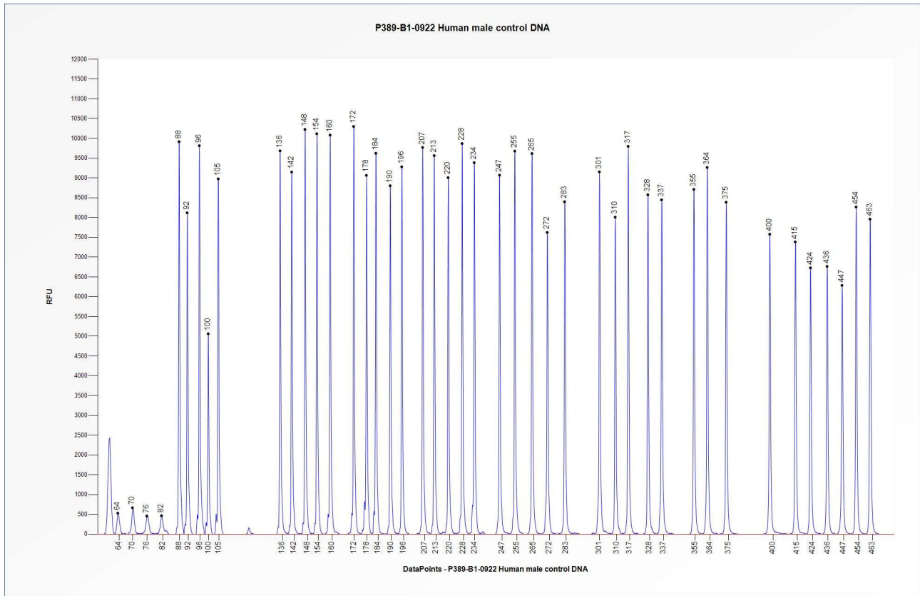
Figure 1. Capillary electrophoresis pattern from a sample of approximately 50 ng human male control DNA analysed with SALSA MLPA Probemix P389 MLL2 (B1-0922).
