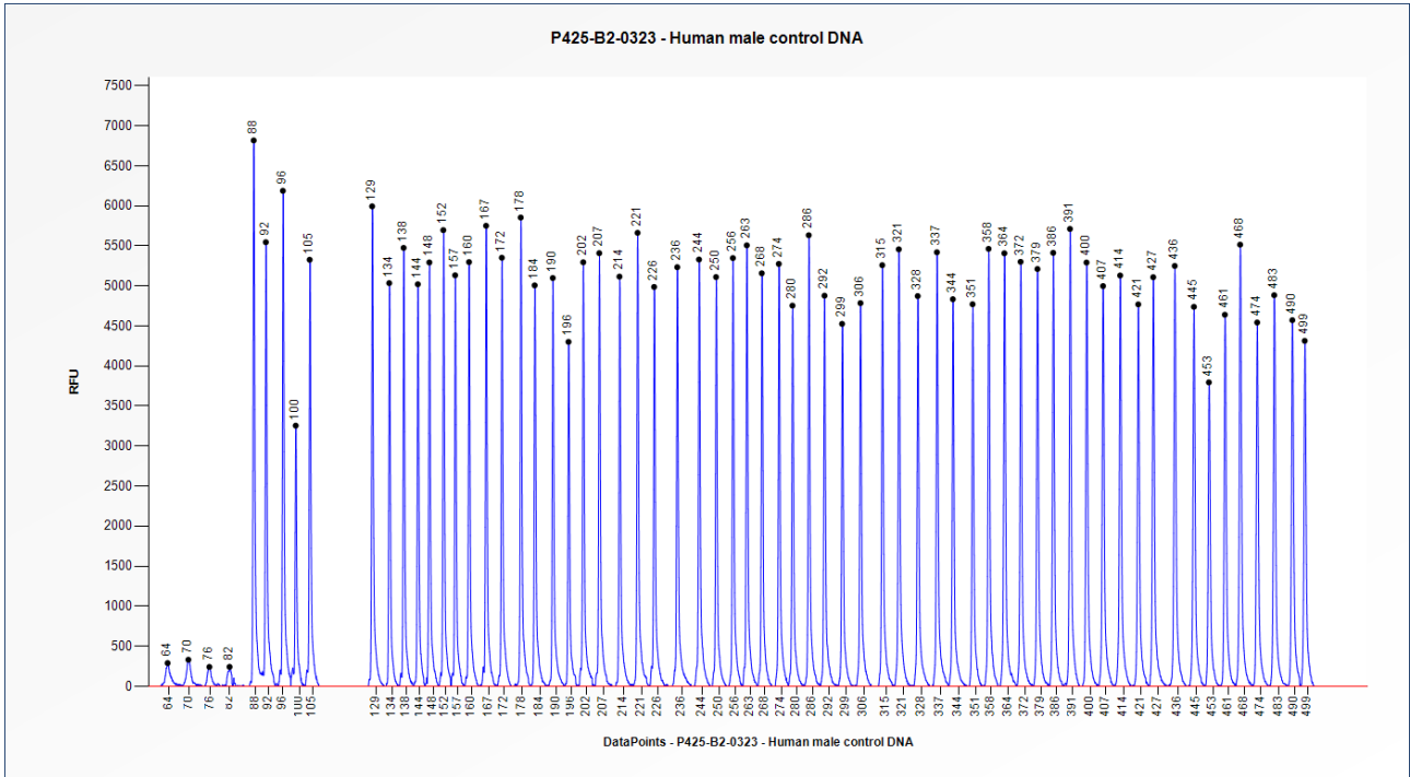
Figure 1. Capillary electrophoresis pattern from a sample of approximately 50 ng human male control DNA analysed with SALSA MLPA Probemix P425 Myeloma (B2-0323).
