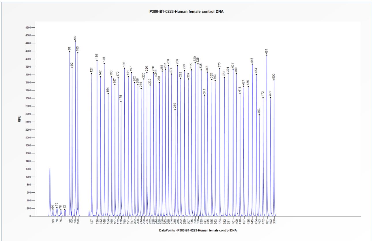
Figure 2. Capillary electrophoresis pattern from a sample of approximately 50 ng human female control DNA analysed with SALSA MLPA Probemix P380 Wilms’ tumour (B1-0223).
