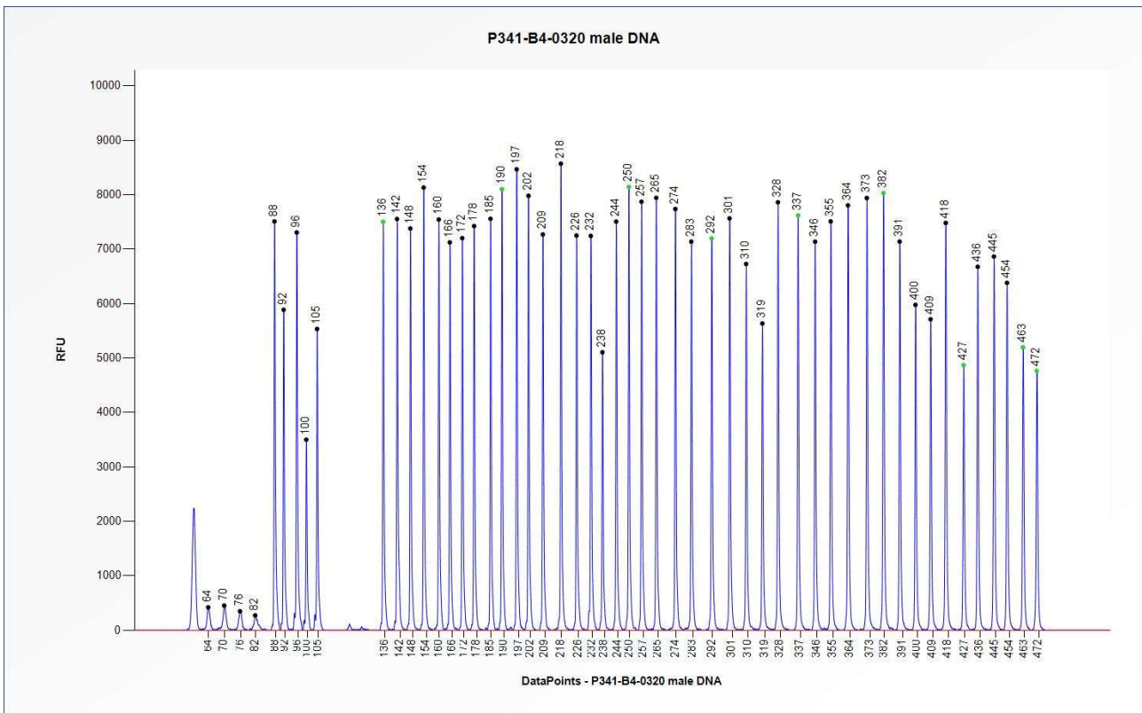
Figure 1. Capillary electrophoresis pattern from a sample of approximately 50 ng human male control DNA analysed with SALSA MLPA Probemix P341 PKHD1 mix 1 (B4-0320).
