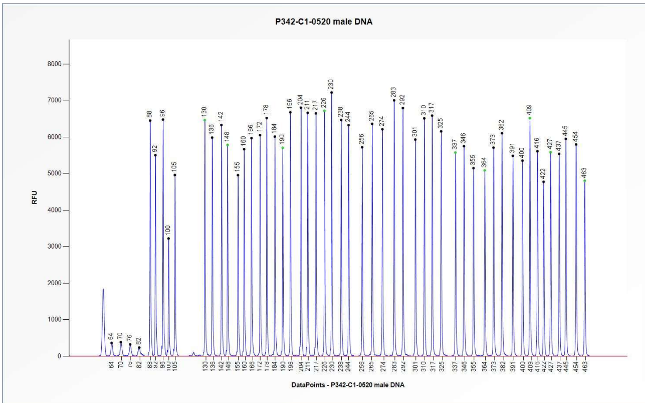
Figure 1. Capillary electrophoresis pattern from a sample of approximately 50 ng human male control DNA analysed with SALSA MLPA Probemix P342 PKHD1 mix 2 (C1-0520).
