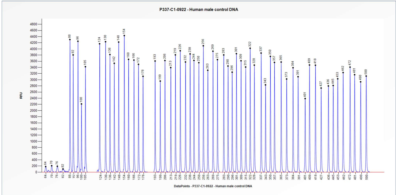
Figure 1. Capillary electrophoresis pattern from a sample of approximately 50 ng human male control DNA analysed with SALSA MLPA Probemix P337 TSC2 Confirmation (C1-0922).
