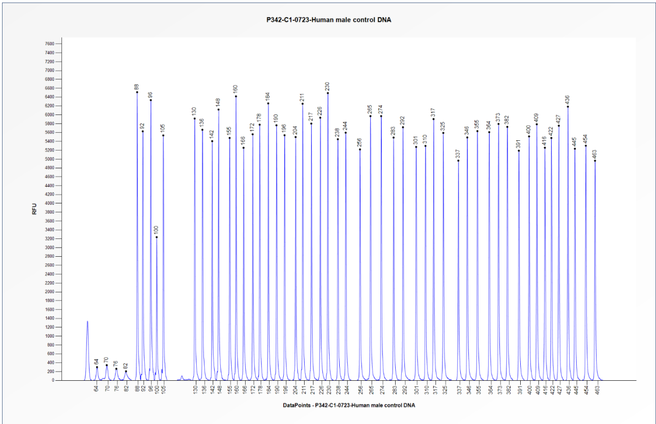
Figure 1. Capillary electrophoresis pattern from a sample of approximately 50 ng human male control DNA analysed with SALSA MLPA Probemix P342 PKHD1 mix 2 (C1-0723).
